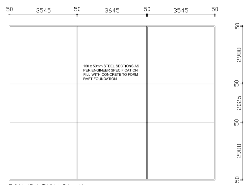
FOUNDATION PLAN Scale 1:100
