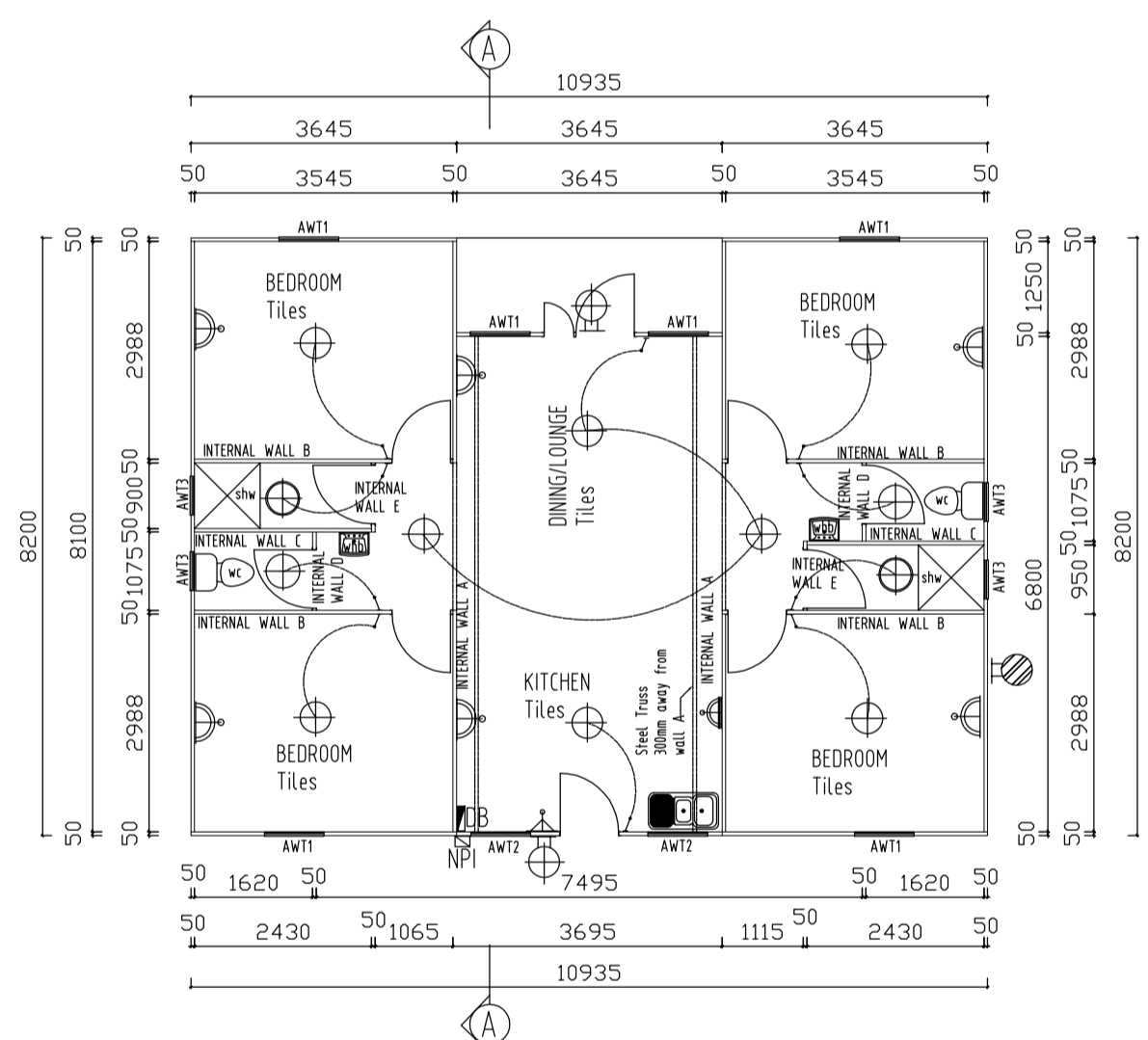
FLOOR PLAN Scale 1:100 (Area 89.6m 2 )
